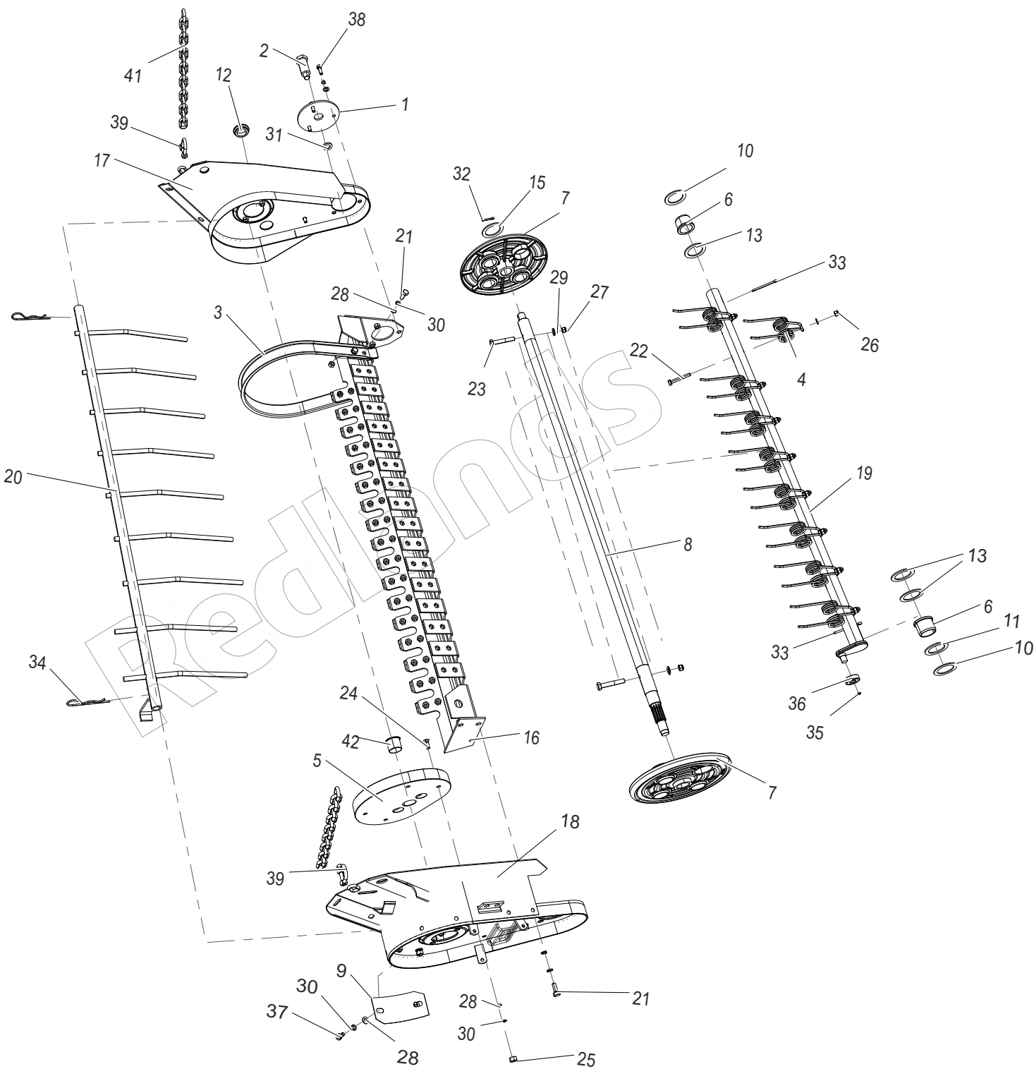
STRAW PICKUP ASSEMBLY
