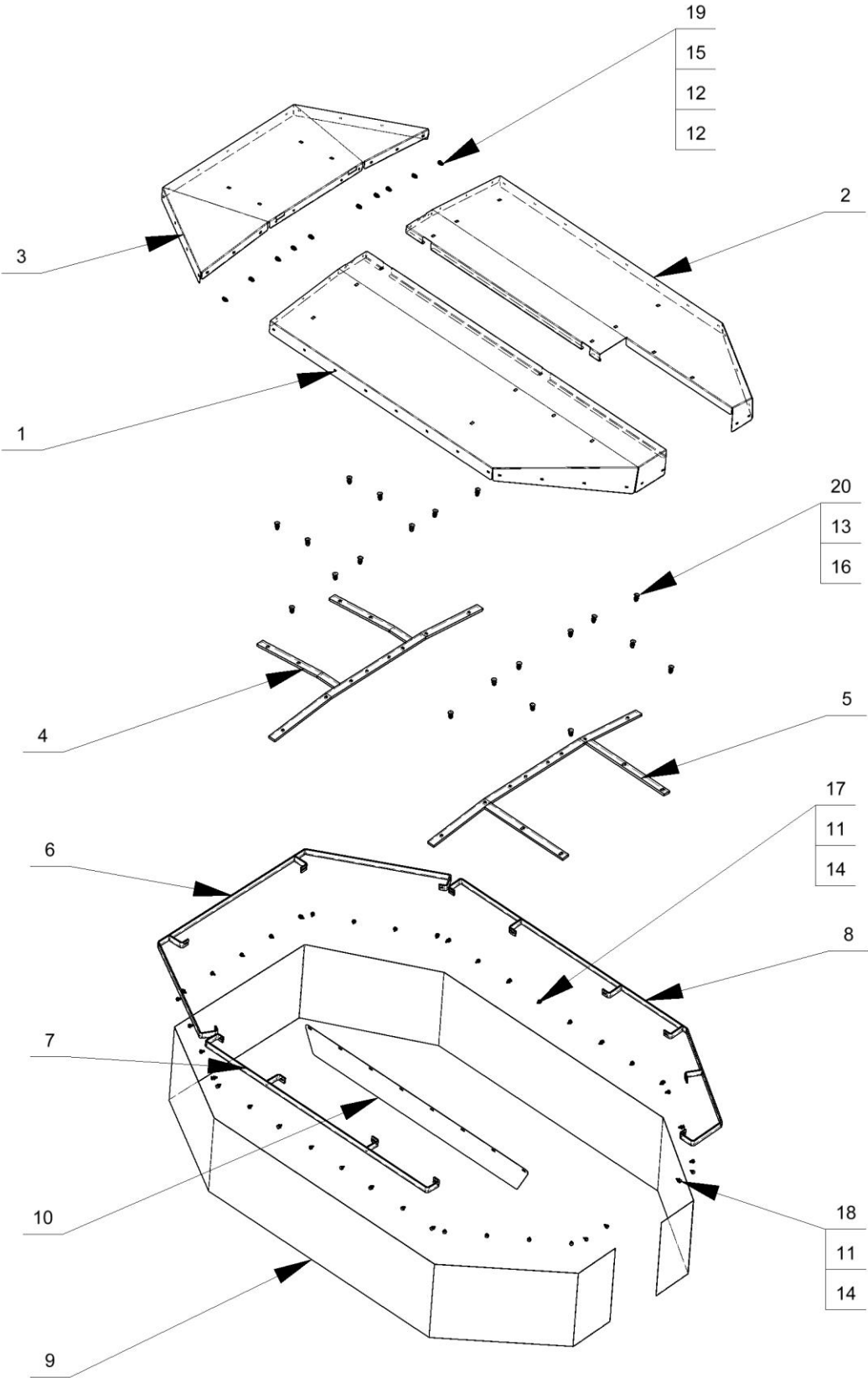
Pic. 5 Cover assembly.
